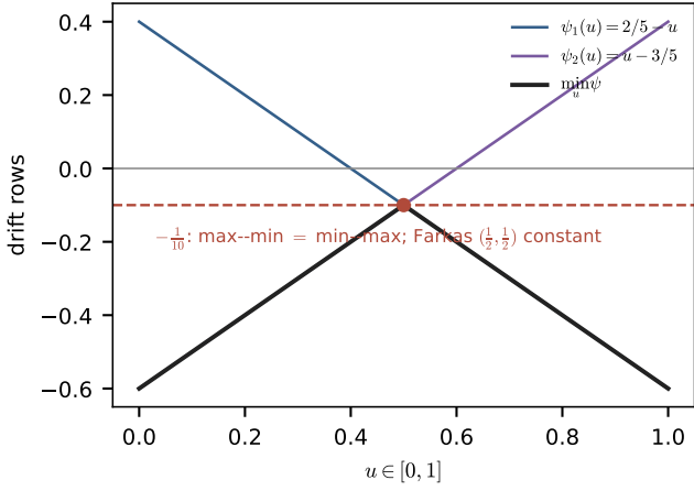
Figure 5: Static duality on the two-floor instance. The two drift rows cross at u = 1/2 ; the max-min equals the min-multiplier maximum at -1/10 , and the normalized Farkas pair (1/2, 1/2) makes the expected drift constant at the value.
